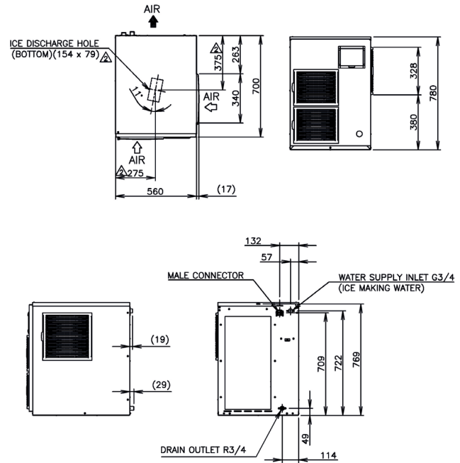
FM-48oAKE-HCN-SB
